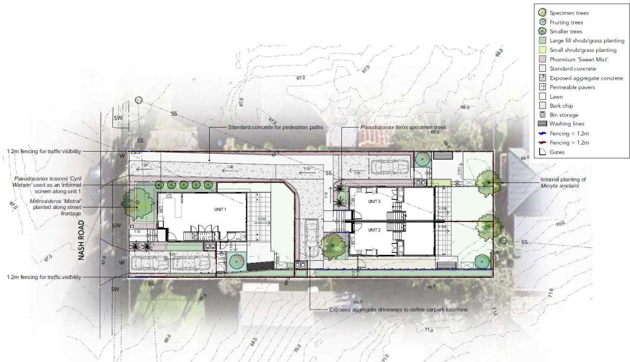
Figure 2: 16 Nash Road, Site Plan
