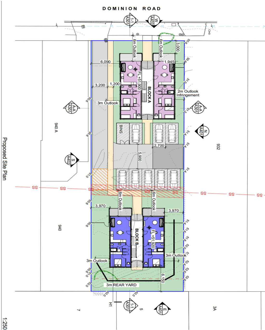
Figure 1 - Site Plan
