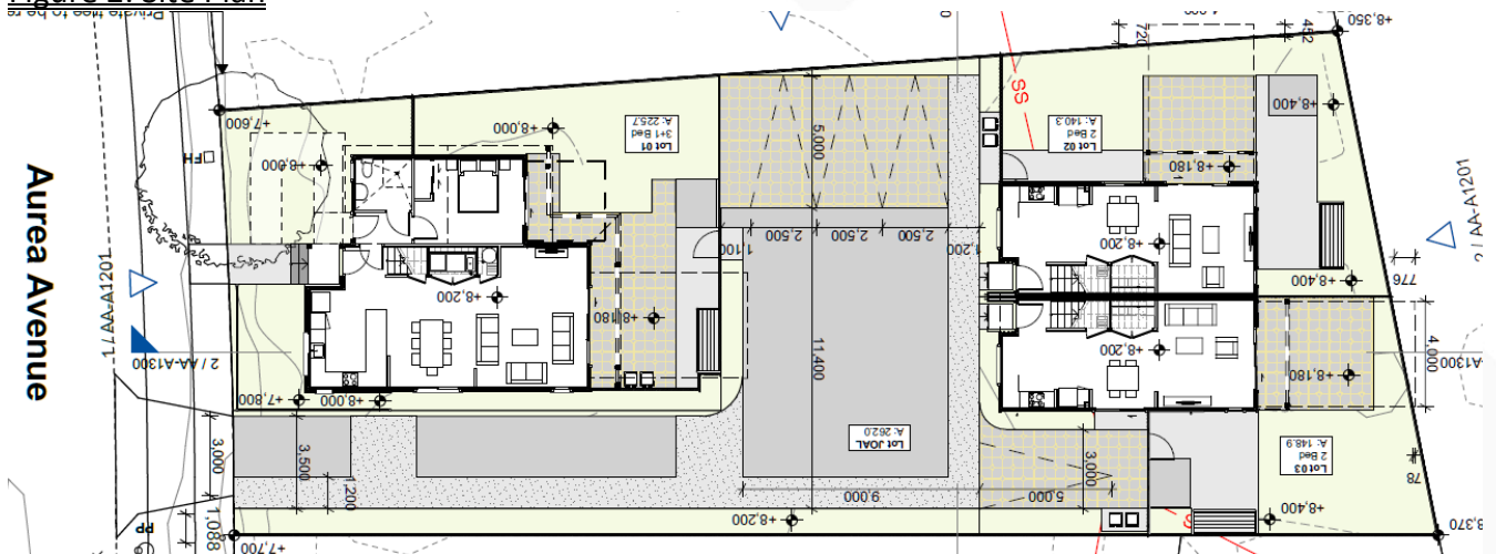
Figure 2: Site Plan
